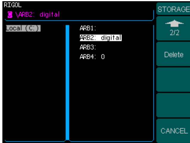
Figure 2-25 File delete
