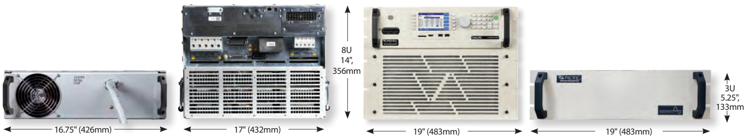
360LMXT Power Source with optional external high range transformer module.
