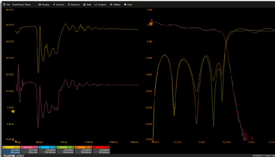
The impedance profile clearly indicates a defective connector in the signal path.
